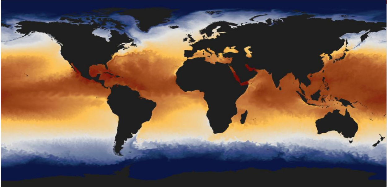
Tidal Elevations
